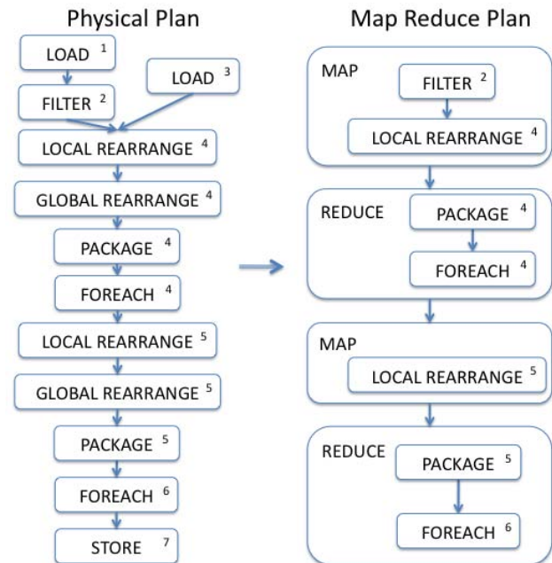
Figure 5: Physical plan to map reduce plan translation.
