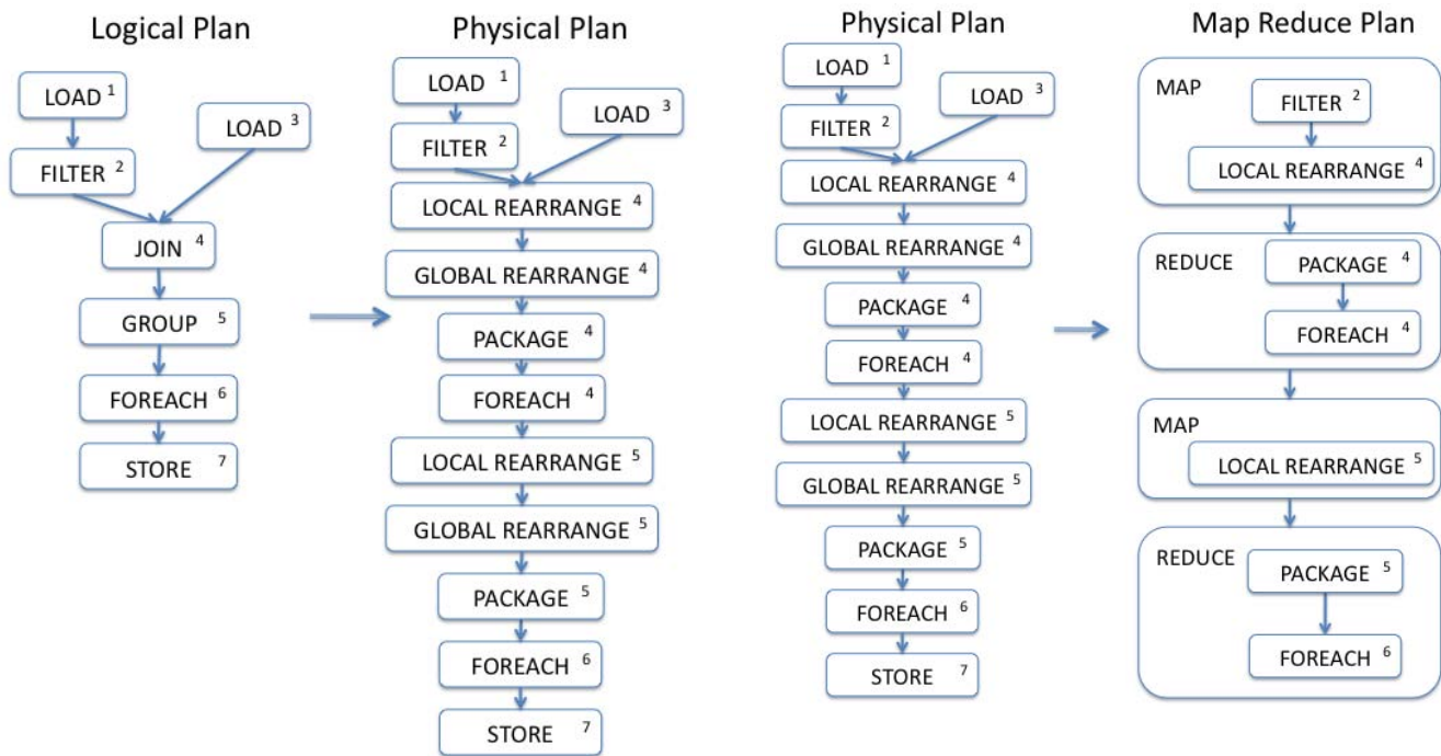
Figure 5: Physical plan to map reduce plan translation.
